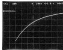
B-1波形 τ:60ms V:20V/Div H:20ms/Div
