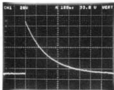
A-1波形 τ:200ms V:20V/Div H:100ms/Div
