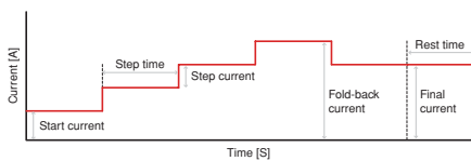
▲ I-V measurement
