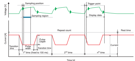
▲ Current interrupt measurement
