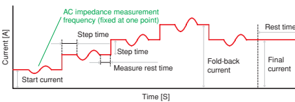
▲ I-V + AC impedance measurement
