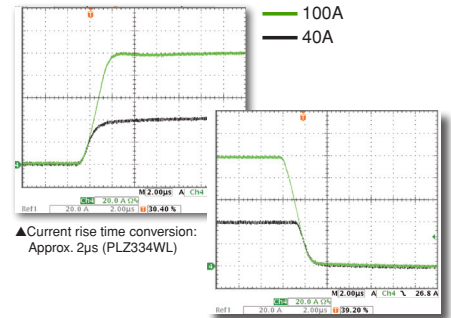
▲ Current rise time conversion: Approx. 2μs (PLZ334WL) ▲ Current fall time conversion: Approx. 2μs (PLZ334WL)
